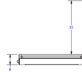
Side View Assembled - Minimum Height Setting
