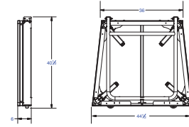
Side View Storage Position (360172 Unit Shown)
