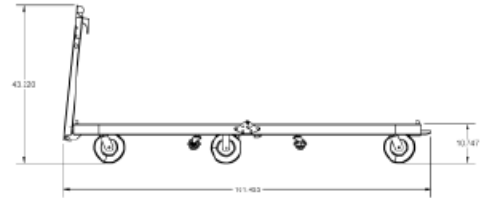
Side View Assembled Position
